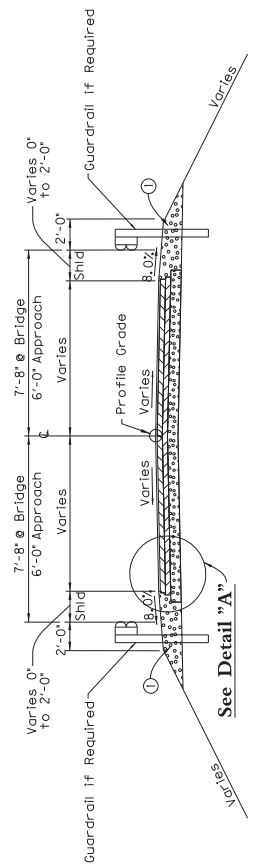
NORMAL SECTION
